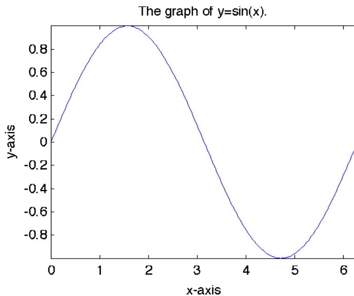
Figure 2.2. The graph of y = \sin x on the interval [0, 2\pi] .
